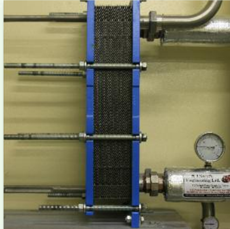
Plate heat exchanger used to cool the milk.
